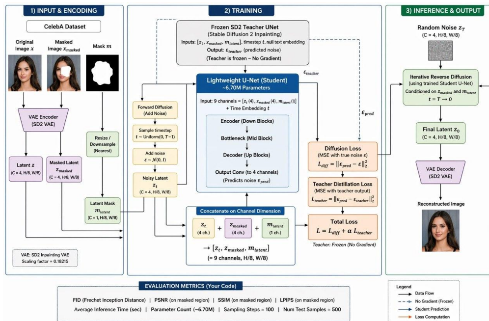
Figure 1 Proposed lightweight latent diffusion inpainting architecture for Student A02.
