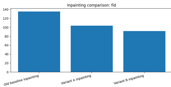
5(a) FID comparison
